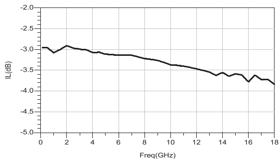
插入损耗
