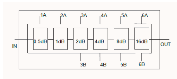
YAT14-00186C1框图
