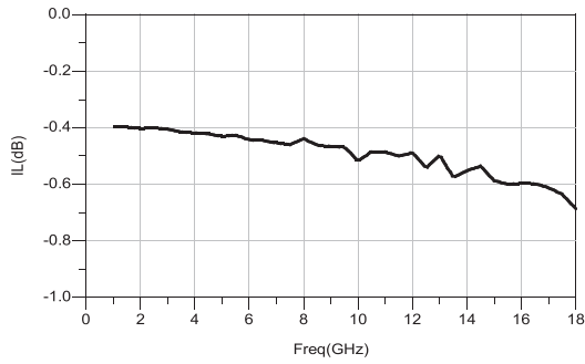
插入损耗
