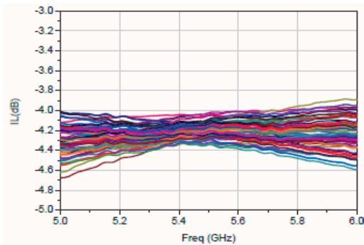
插入损耗
