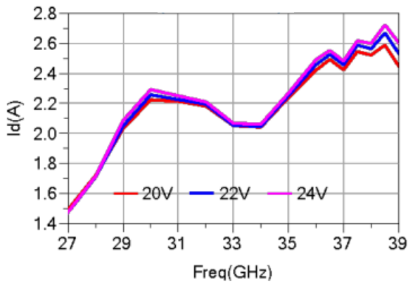
饱和电流 vs. 频率 ( P_{in} = 26\text{dBm} )
