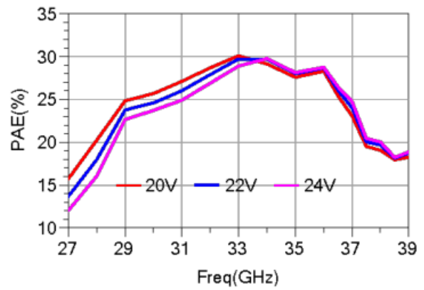
附加效率 vs. 频率 ( P_{in} = 26\text{dBm} )
