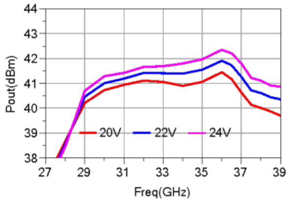
饱和输出功率 vs. 频率 ( P_{in} = 26\text{dBm} )
