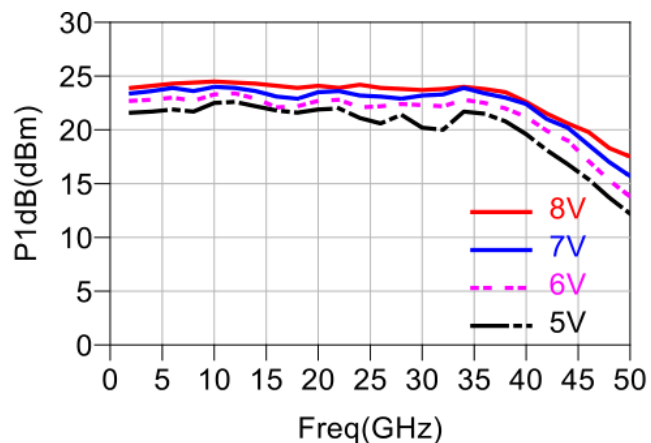
P1dB vs.频率@T A =25°C
