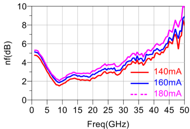
噪声系数vs.频率@T A =25°C
