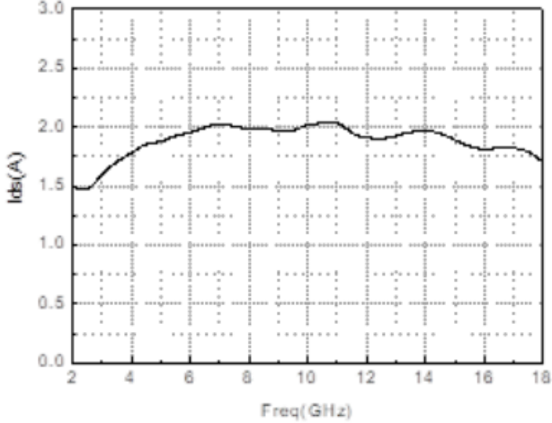
动态漏极电流 vs. 频率 ( P_{in} = 28\text{dBm} )
