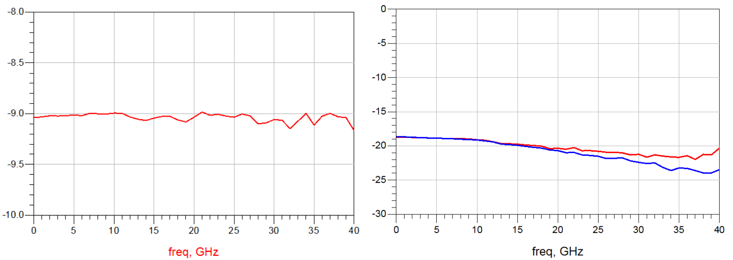
插入损耗
