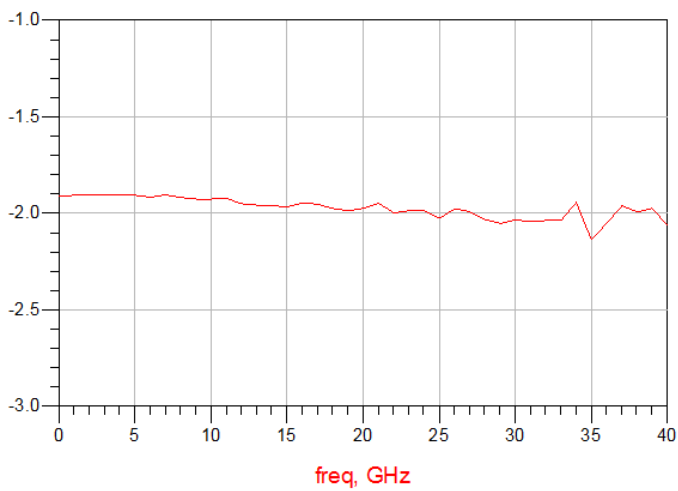
插入损耗
