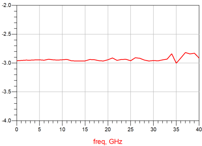
插入损耗
