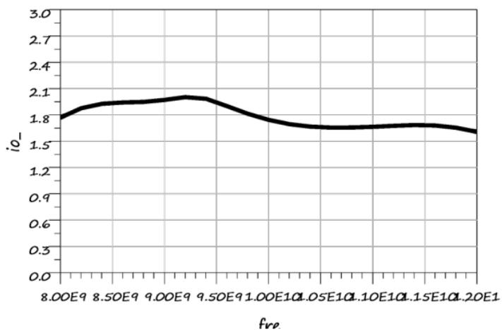
动态漏极电流 vs. 频率 ( P_{in} = 19\text{dBm} )
