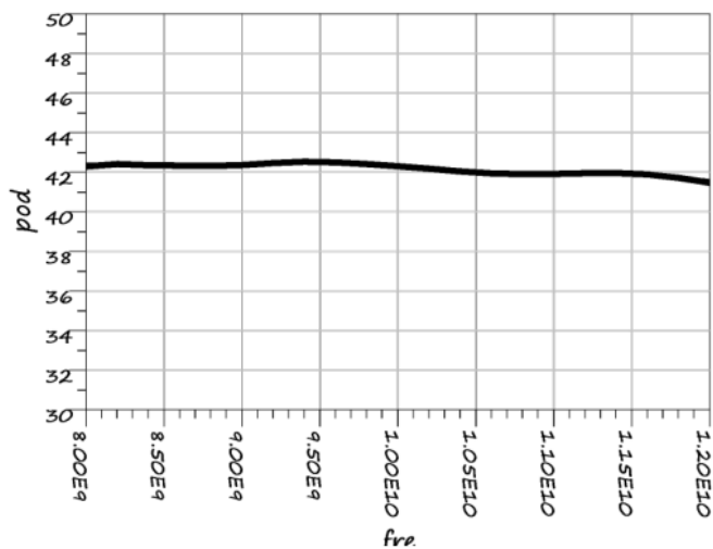
饱和输出功率 vs. 频率 ( P_{in} = 19\text{dBm} )
