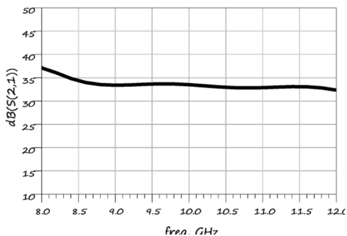
线性增益 vs. 频率 ( P_{in} = -10\text{dBm} )
