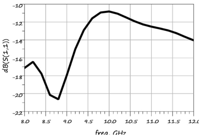
输入驻波 vs. 频率 ( P_{in} = -10\text{dBm} )
