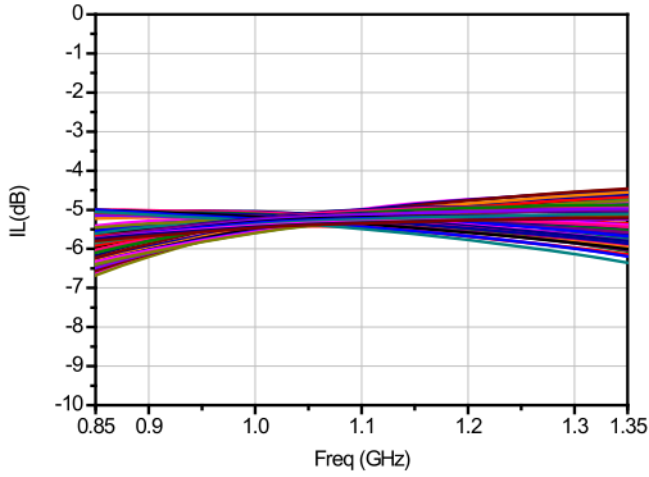
插入损耗
