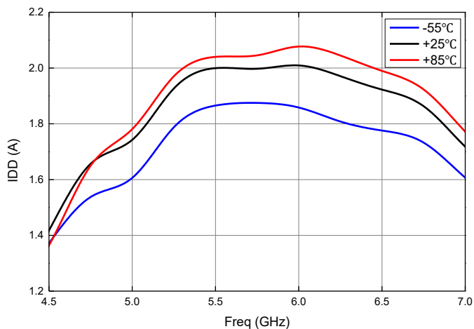
动态电流 (CW)
